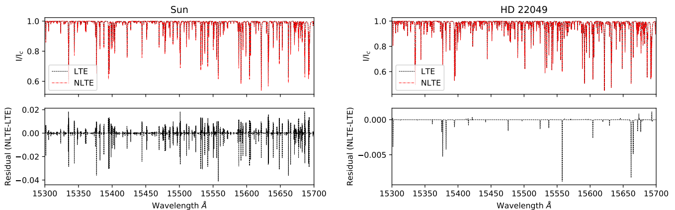
Fig. 1: Investigation of the influence of NLTE effects in spectra of stars with different stellar parameters in the H-band. Left : synthetic spectra for solar parameters; right : calculations for parameters of HD 22049, one of the coolest stars in our sample. Top panels show synthetic spectra for LTE (solid black line) and NLTE (dashed red line) while the bottom panels show the difference between the NLTE and LTE synthetic spectra.
