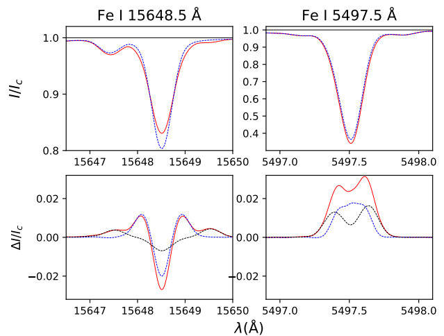
Fig. 8: Impact of a magnetic field distribution with multiple components on the theoretical profiles of the magnetically sensitive lines Fe I 15648.5 \text{ \AA} (this study) and Fe I 5497.5 \text{ \AA} (Kochukhov et al. 2020) for a star with solar parameters rotating with a v \sin i of 5 \text{ km s}^{-1} . In this case, the magnetic field distribution is composed of 0, 1, and 3 kG fields covering 75, 20, and 5% of the stellar surface respectively. Top : non-magnetic spectra in dashed blue and the combined magnetic spectra in red. Bottom : difference between the magnetic and non-magnetic spectra in red, contribution to this difference by the 1 and 3 kG field is shown in dashed blue and dashed black respectively.
