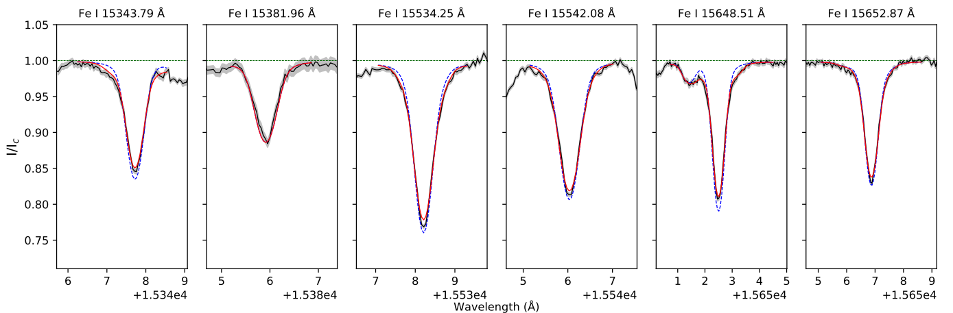
Fig. 2: Two-component model fit to the spectrum of HD 20630 showing the observed spectra in black, the best fit synthetic model in red and the synthetic model with the same stellar parameters but without magnetic field in dashed blue. The continuum is also shown as the yellow dotted line.
