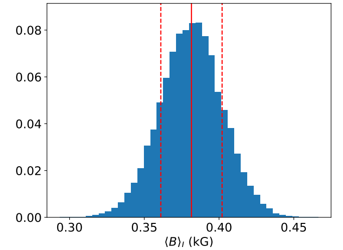
Fig. 4: Same as Fig 3 but for the multi-component model applied to HD 20630.
