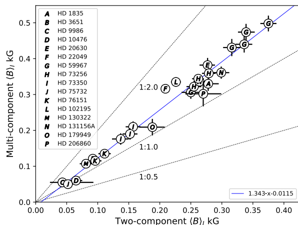
Fig. 5: Comparison between the magnetic field values obtained using different model prescriptions of Eq. (1) and (2). The solid blue line represents a linear fit to the data.
