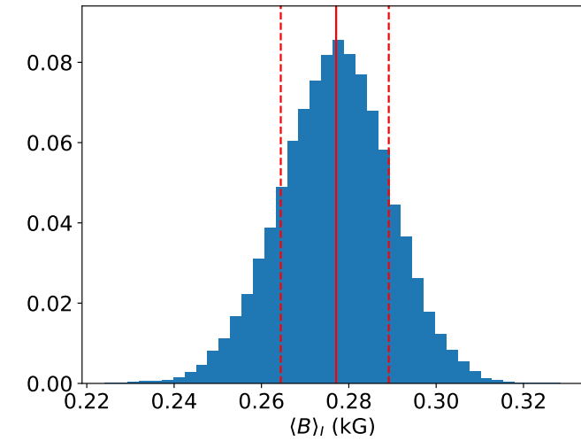
Fig. 3: Top. Posterior distributions of the parameters in the sampling of HD 20630 using the two-component model. Bottom. Posterior distribution of the average magnetic field strength \langle B \rangle_I given by Bf_B .
