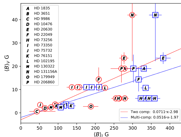
Fig. 6: Mean strengths of the large- and small-scale fields from Table 1 and 3 respectively. Red circles represents the two-component results. Blue squares represent multi-component results that are significantly different compared to their two-component counterpart. Dashed lines show linear fits, red for the two-component model and blue for the multi-component model. Uncertainties in \langle B \rangle_V represent scatter in the ZDI results corresponding to different observing epochs. Stellar labels are the same as in Fig. 5
