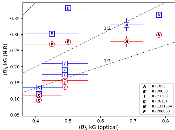
Fig. 7: Relationship between the small-scale magnetic field strength measured at different wavelengths. The y-axis corresponds to the average magnetic field strength obtained in this study while the x-axis shows the optical measurements taken from Kochukhov et al. (2020). Black dotted lines represent fractions between the two results. Stellar labels are the same as in Fig. 5 and 6.
